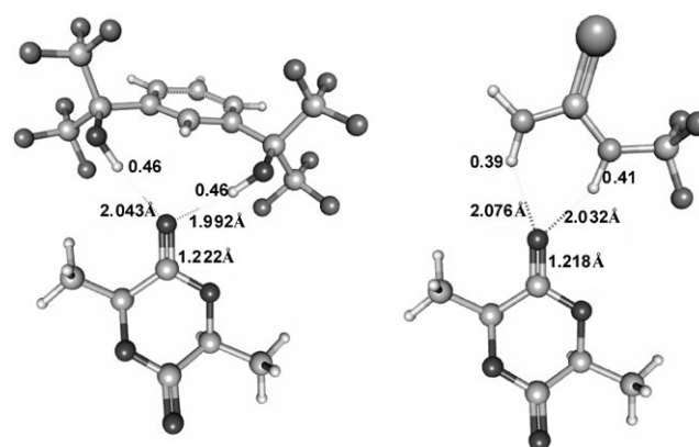
Figure 2. Comparison of L-lactide 10a adduct with 6c and model thiourea catalysts: hydrogen-bond lengths, carbonyl bond lengths, and partial charges on the hydrogen atoms that participate in hydrogen bonding to the oxygen atom of the carbonyl group.
