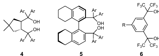
Scheme 2. Representative structures of diol hydrogen-bonding donor catalysts.
