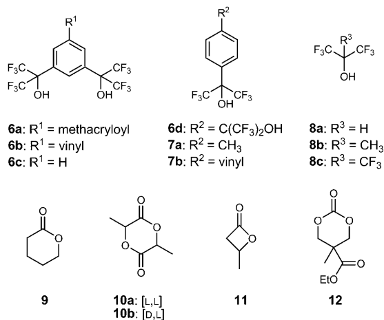
Scheme 3. Double- ( 6a–d ) and single- ( 7a,b and 8a–c ) hydrogen-bonding catalysts and cyclic esters ( 9 , 10a,b , 11 ), and carbonate ( 12 ).
