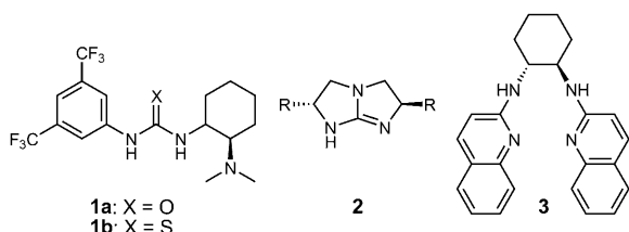
Scheme 1. Representative structures of urea 1 (X=O), thiourea 1 (X=S), guanidinium 2 , and amidinium ions 3 (charges omitted).
