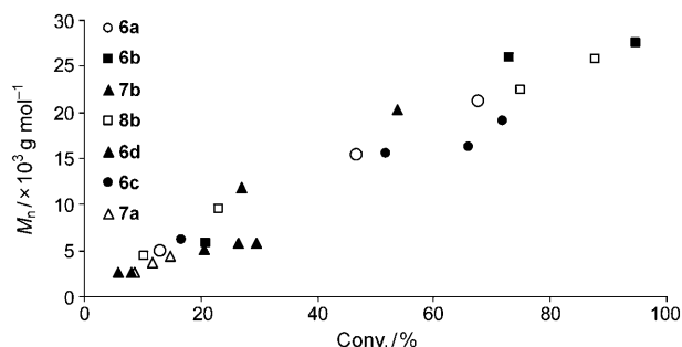
Figure 4. Plot of M_n (estimated by GPC) versus LA conversion (estimated by ^1\text{H} NMR; \text{CH}_2\text{Cl}_2 , RT, [\mathbf{10a}]_0 = 1\text{ M} , [\mathbf{10a}]/[\text{catalyst}]/[\text{BnOH}]/[\text{S}] = 200/5/1/1 ).
