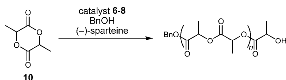
Scheme 4. ROP of a lactide by HFA catalysts.
