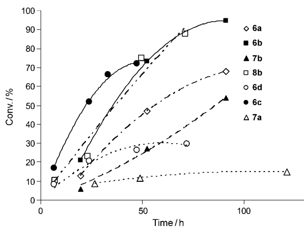
Figure 3. Time-conversion curves obtained from ROPs of LA in \text{CH}_2\text{Cl}_2 at RT ( [\mathbf{10a}]/[\text{catalyst}]/[\text{BnOH}]/[\text{S}] = 200:5:1:1 ; [\mathbf{10a}]_0 = 1\text{ M} ).
